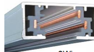
3Wires
