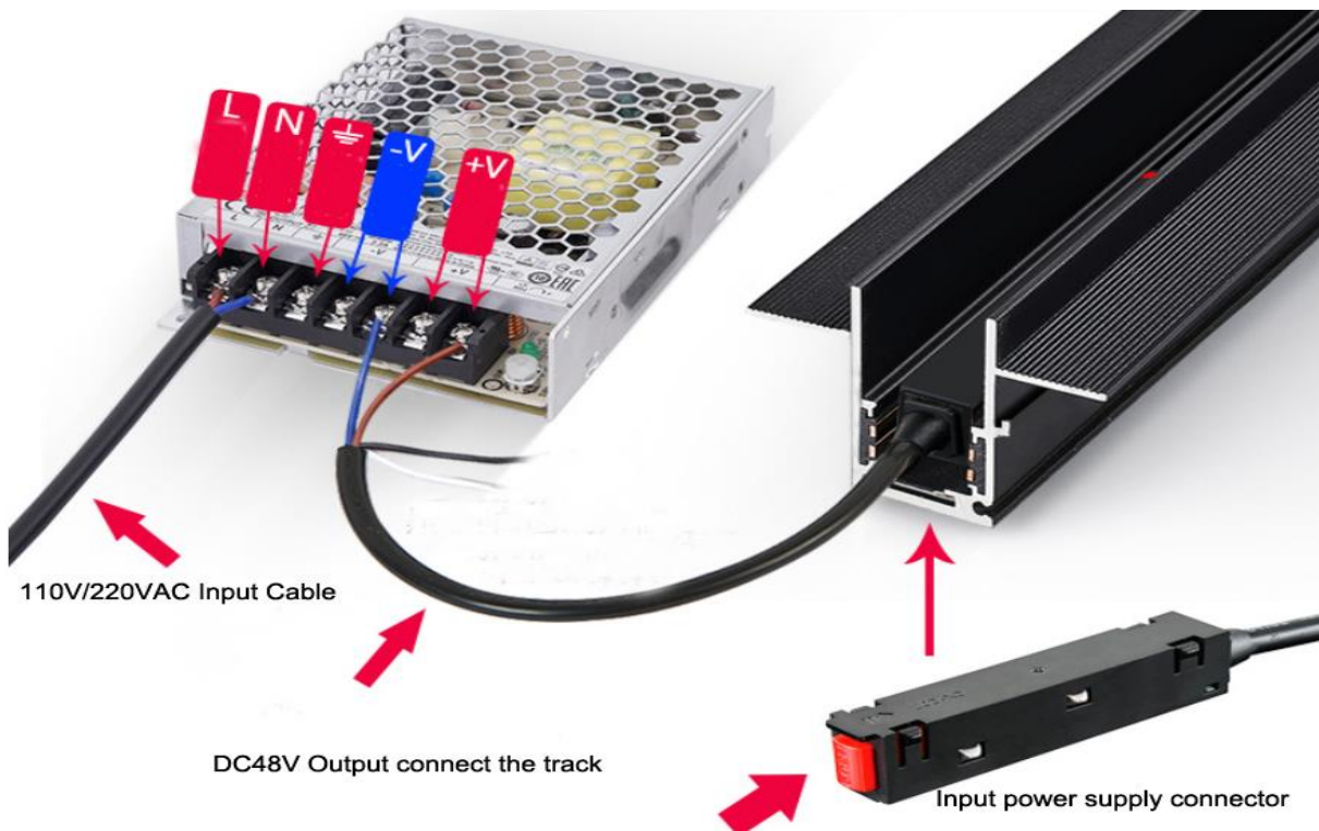
DC48V Power supply works with Input power supply connector
